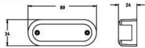
ME 6 LED, 24V
